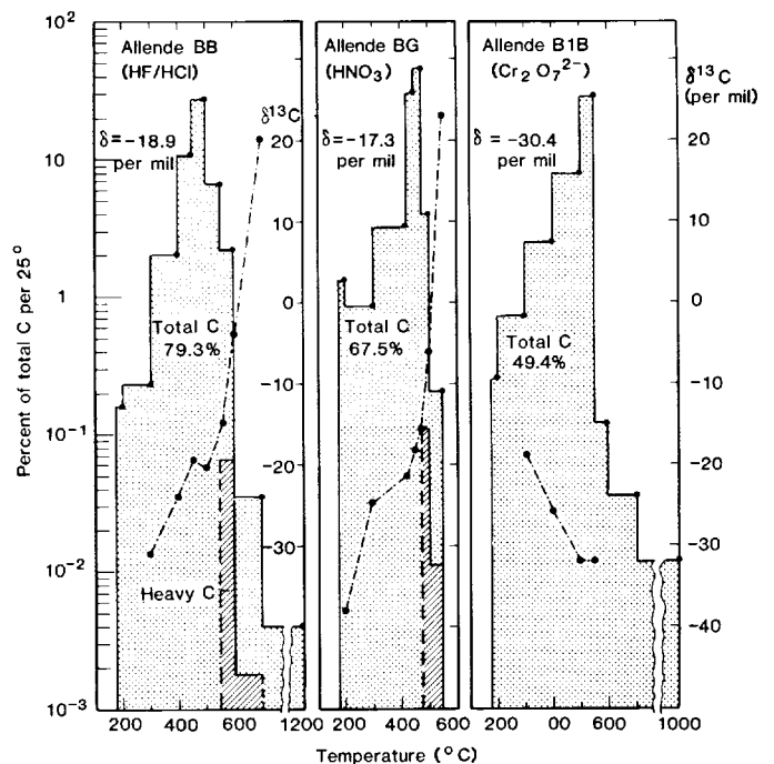
Fig. 1 (top left). Carbon released by stepped combustion of the Murchison meteorite before and after treatment with \text{H}_3\text{PO}_4 . Dot-dashed line gives isotopic composition. In the bulk meteorite, the major part of the carbon, evolving to 550^\circ\text{C} , is isotopically normal, but the last 6 percent is isotopically heavy. At least the portion between 600^\circ and 850^\circ\text{C} must be due mainly to carbonates, which are known to decompose in this interval and have \delta^{13}\text{C} of +35 to +51 per mil. Treatment with \text{H}_3\text{PO}_4 removes 86 percent of the sample, including carbonates and water-soluble organic compounds, but still leaves a small (0.51 percent), very heavy carbon component that is released mainly between 1000^\circ and 1200^\circ\text{C} . For the \text{H}_3\text{PO}_4 -treated sample, fractions from 700^\circ\text{C} upward were blank corrected. Fig. 2 (top right). Two demineralized samples, from which most of the carbon was removed by \text{NaOCl} and \text{H}_2\text{O}_2 , are about 10^3 -fold enriched in heavy carbon and show \delta^{13}\text{C} up to +1100 per mil (or up to +883 per mil before blank correction). The release curve of heavy carbon in 2C10m is very wide and bimodal, suggesting that at least two types of heavy carbon are present. They may be associated with Ne-E(L) and s -Xe. Sample 2C10f, which contains large amounts of CCFXe, also shows a characteristic light carbon component ( -32 to -38 per mil) at 500^\circ\text{C} .
