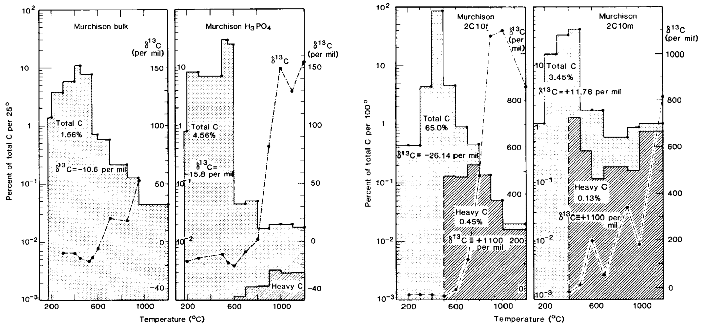
Fig. 1 (top left). Carbon released by stepped combustion of the Murchison meteorite before and after treatment with \text{H}_3\text{PO}_4 . Dot-dashed line gives isotopic composition. In the bulk meteorite, the major part of the carbon, evolving to 550^\circ\text{C} , is isotopically normal, but the last 6 percent is isotopically heavy. At least the portion between 600^\circ and 850^\circ\text{C} must be due mainly to carbonates, which are known to decompose in this interval and have \delta^{13}\text{C} of +35 to +51 per mil. Treatment with \text{H}_3\text{PO}_4 removes 86 percent of the sample, including carbonates and water-soluble organic compounds, but still leaves a small (0.51 percent), very heavy carbon component that is released mainly between 1000^\circ and 1200^\circ\text{C} . For the \text{H}_3\text{PO}_4 -treated sample, fractions from 700^\circ\text{C} upward were blank corrected. Fig. 2 (top right). Two demineralized samples, from which most of the carbon was removed by \text{NaOCl} and \text{H}_2\text{O}_2 , are about 10^3 -fold enriched in heavy carbon and show \delta^{13}\text{C} up to +1100 per mil (or up to +883 per mil before blank correction). The release curve of heavy carbon in 2C10m is very wide and bimodal, suggesting that at least two types of heavy carbon are present. They may be associated with Ne-E(L) and s -Xe. Sample 2C10f, which contains large amounts of CCFXe, also shows a characteristic light carbon component ( -32 to -38 per mil) at 500^\circ\text{C} .
