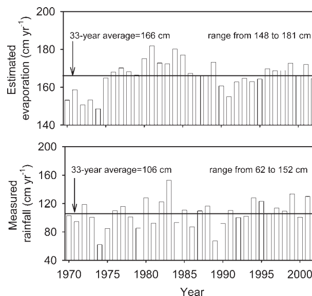
Fig. 4. Long-term estimates of annual evaporation from Florida Bay based upon temperature records from Flamingo, Royal Palm, and Tavernier from 1970 to 2002, and NOAA Division 7 rainfall over the same time period. Note the scales are different between the two graphs.
